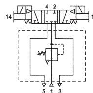
Со mmon port regulator with 4-way, 3-position APB valve
